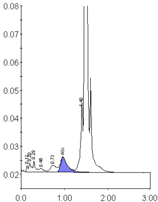
Peak table - ID: 10513534
